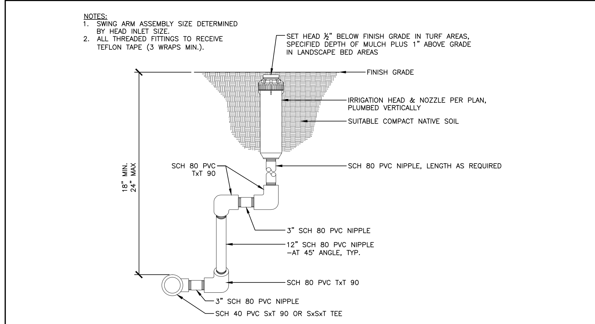
① TYPICAL HEAD & SWING ARM ASSEMBLY NOT TO SCALE
